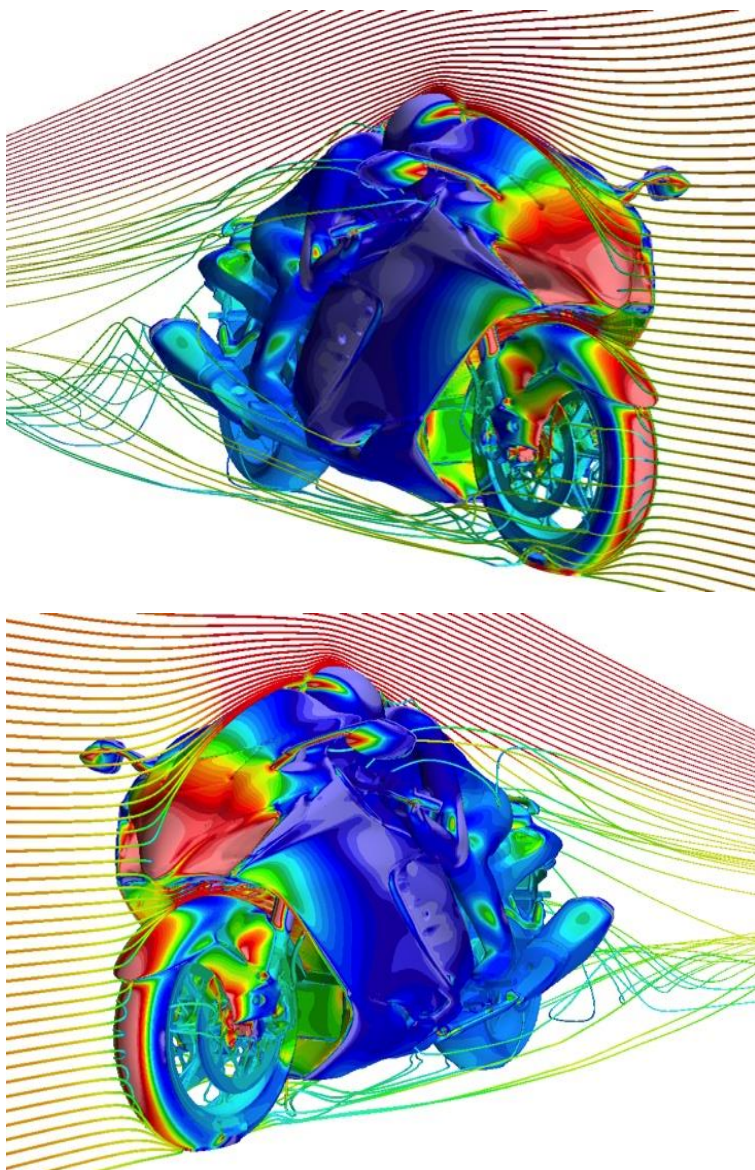
Pressure distribution / velocity distribution chart
