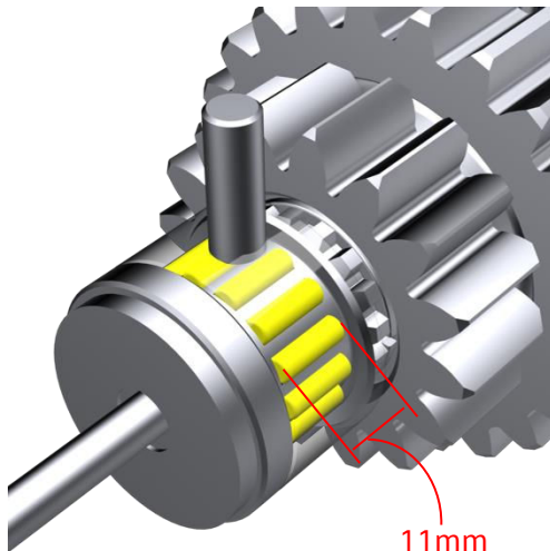
Previous needle bearing
