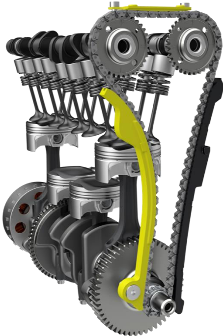
New cam chain tensioner
