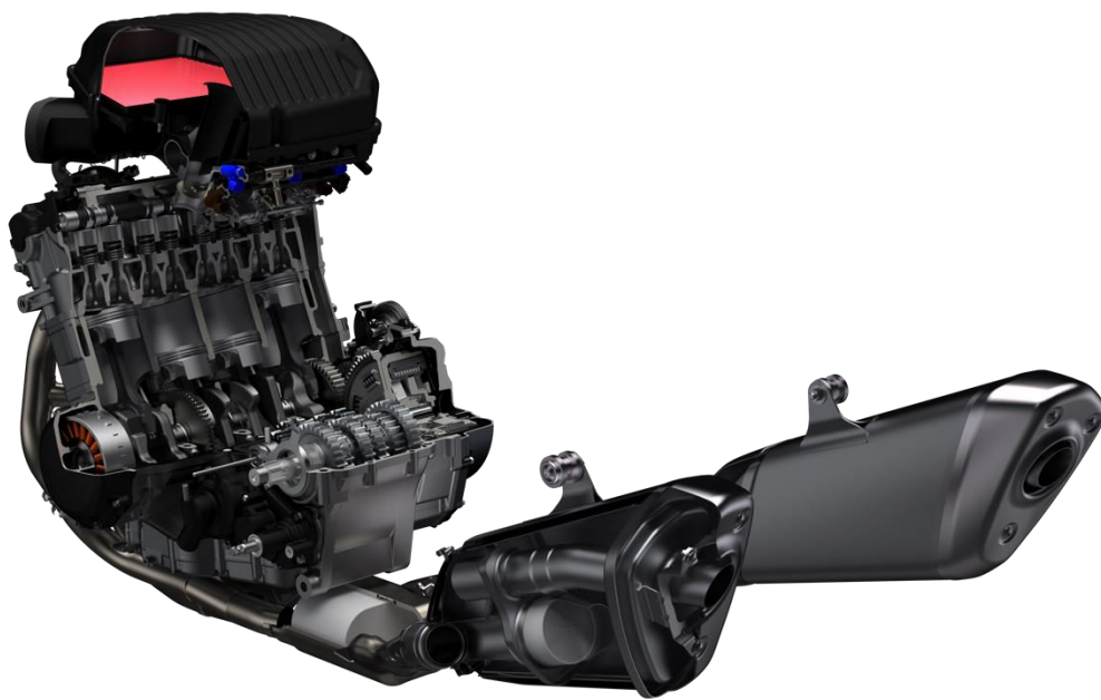
Engine cutaway
