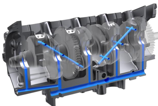
New oil passages
