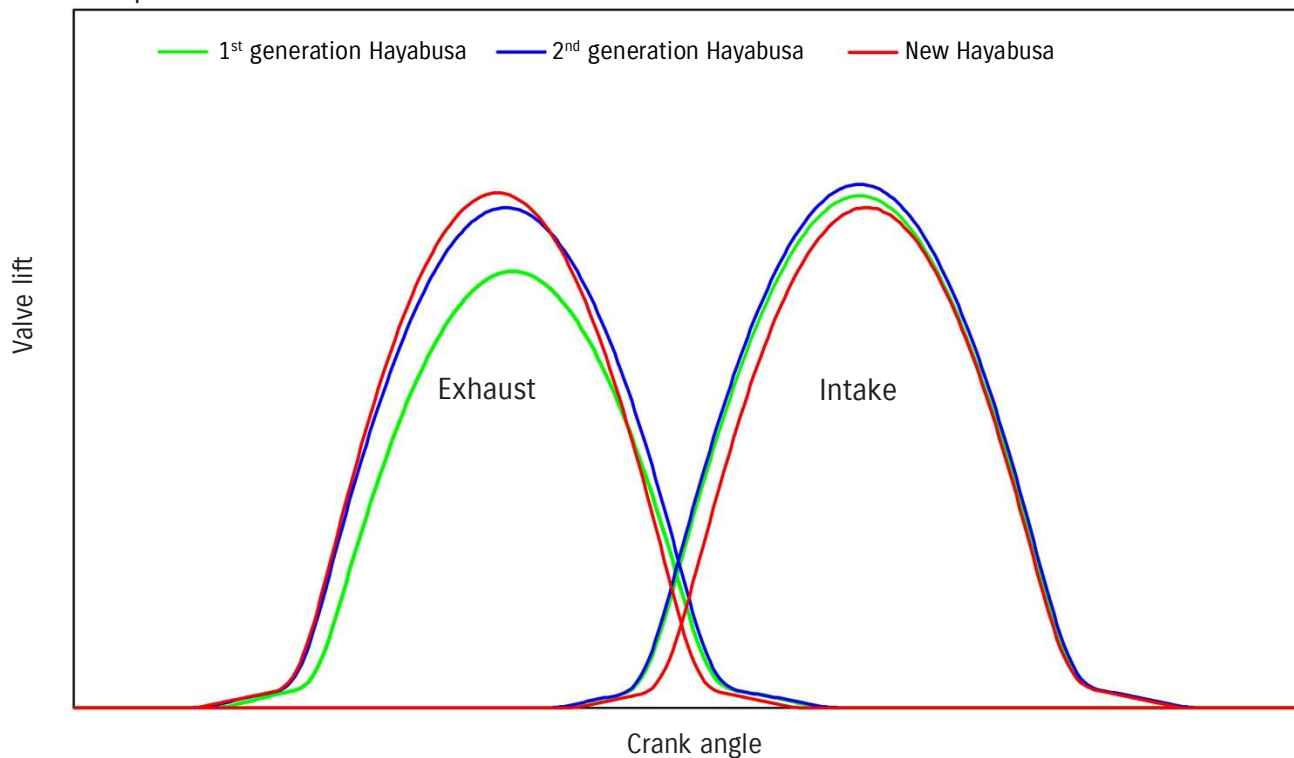
Cam profile
