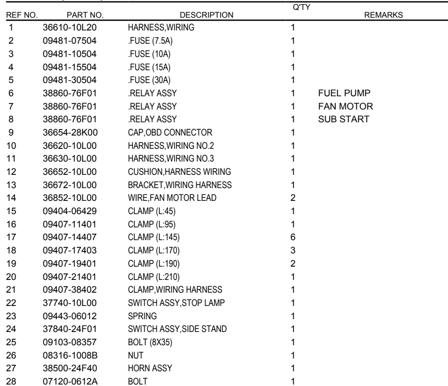
FIG.350A (1-D-13) WIRING HARNESS
